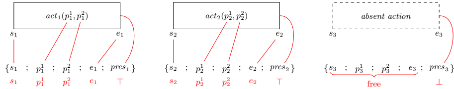
Fig. 1: Relation between the solution plan actions and the CSP action variables
