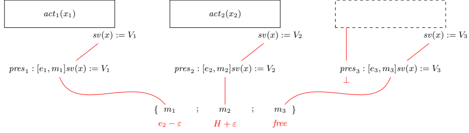
Fig. 3: Relation between the solution plan assign effects and the CSP mutex variables
